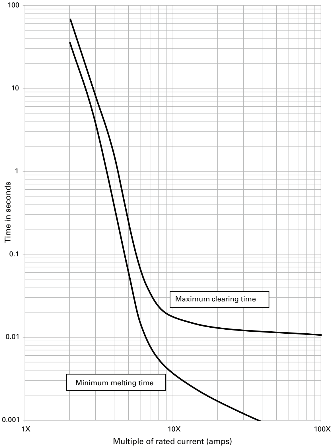
25 mm diameter DC minimum melt / maximum clearing time-current curves — multiple of rated current For catalog numbers EV25-175 to EV25-250 amp fuses supplied via DC rectifier @ 500 Vdc and time constant (L/R) 2 ms ± 0.5 ms
