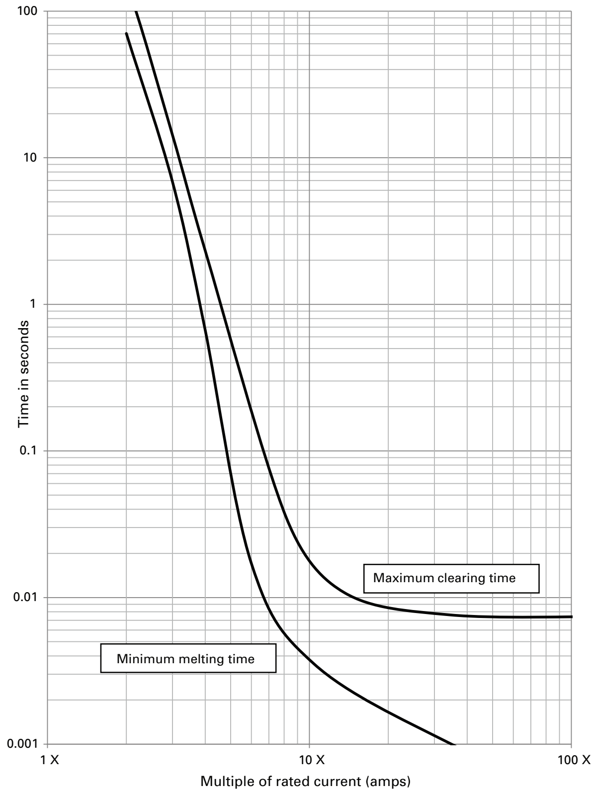
20 mm diameter DC minimum melt / maximum clearing time-current curves — multiple of rated current For catalog numbers EV20-125 to EV20-150 amp fuses supplied via DC rectifier @ 500 Vdc and time constant (L/R) 2 ms ± 0.5 ms
